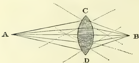
Double Convex Lens.
